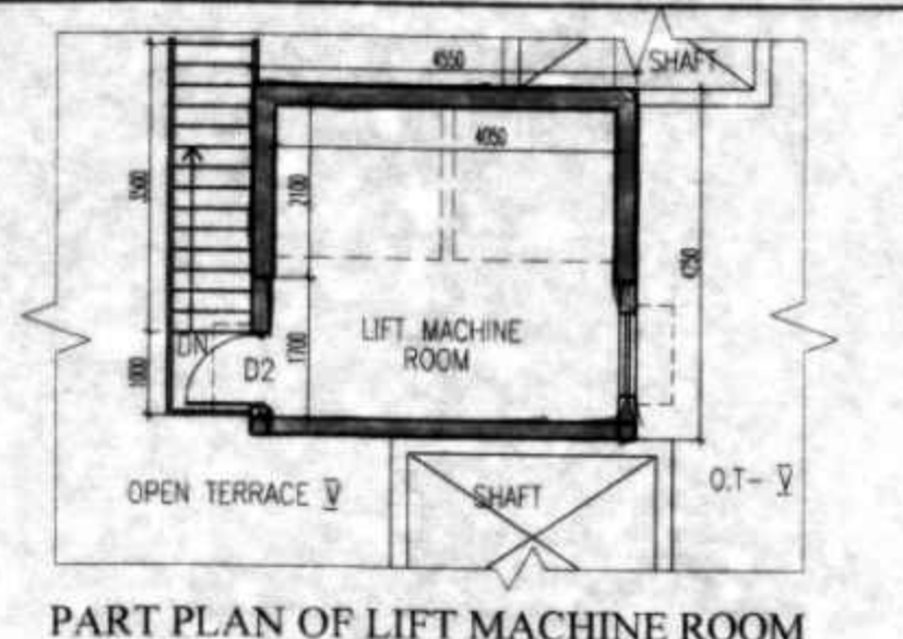
PART PLAN OF LIFT MACHINE ROOM
