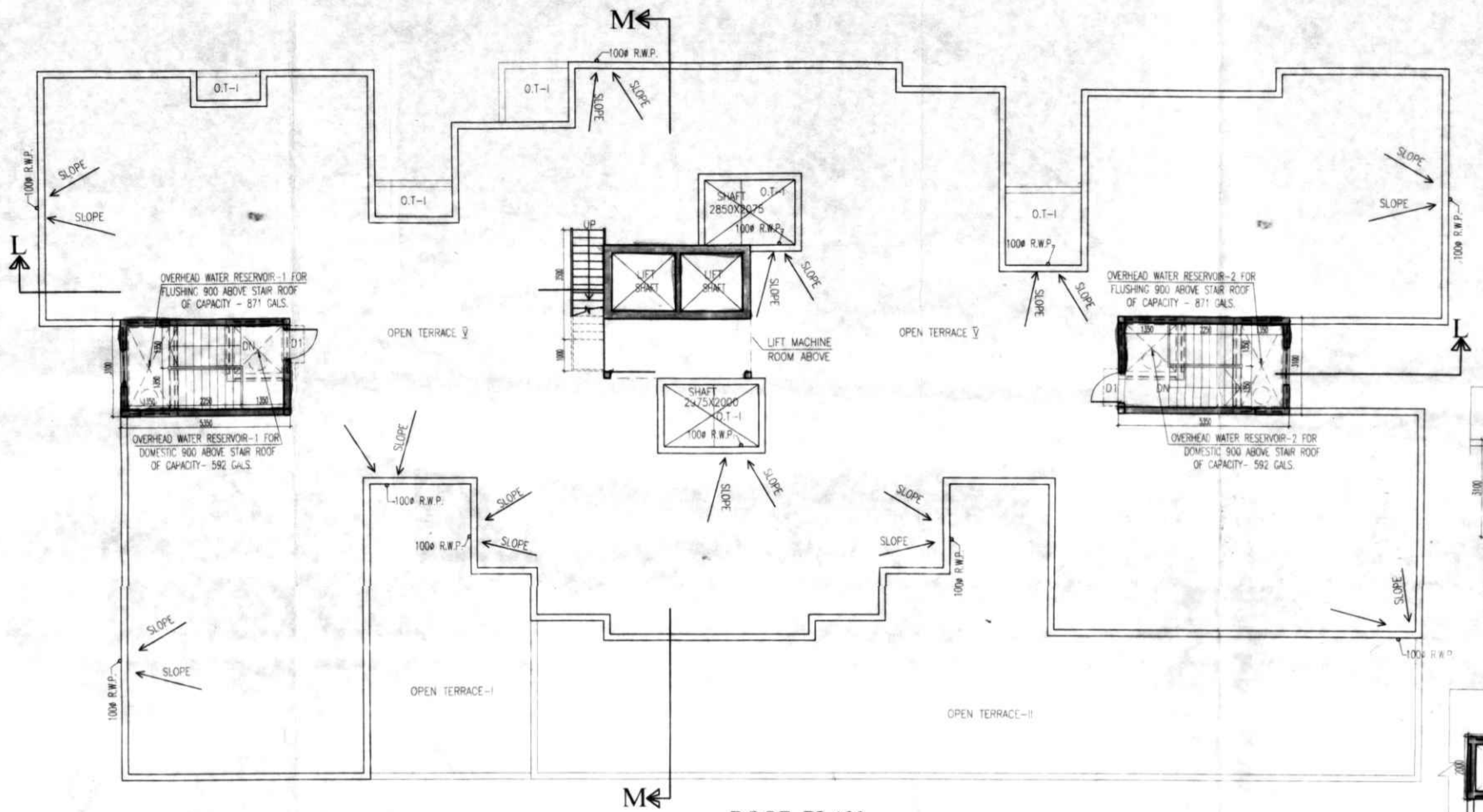
ROOF PLAN
