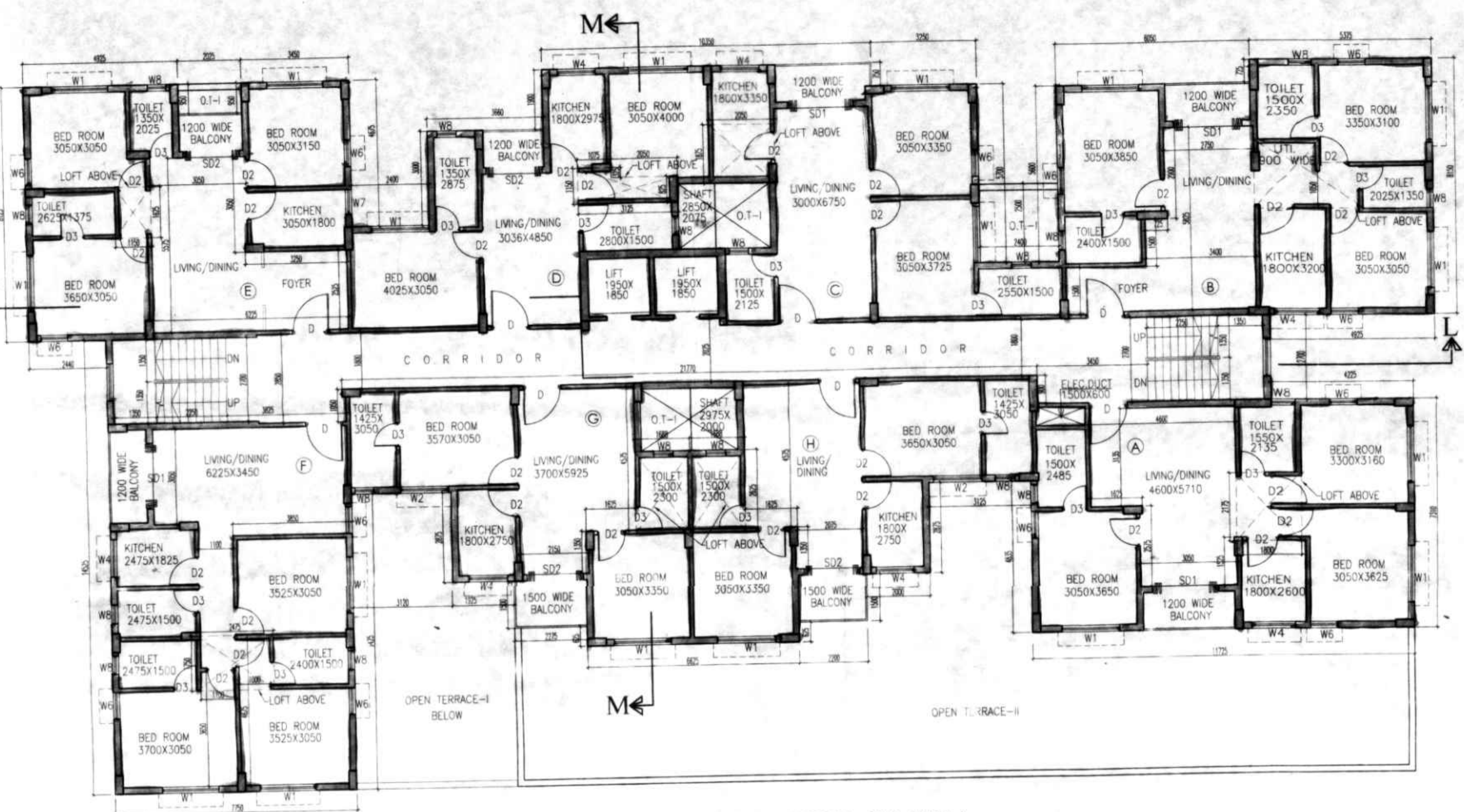
TYPICAL FLOOR PLAN (2ND. TO 4TH.)
